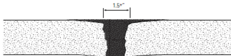
MASTIC WIDE CRACK REPAIR
